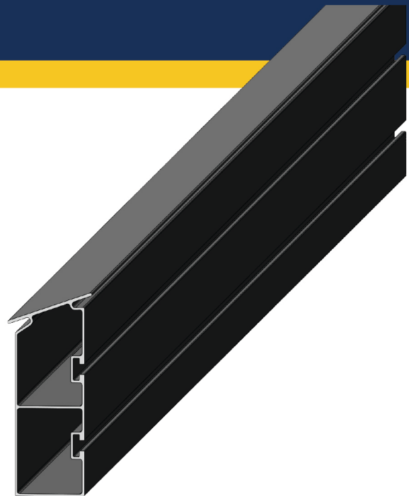
Boat Lift Bunk with Integral T-Slot Nonprovisional 18/418,873
