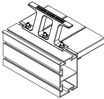
CLEAT ASSEMBLY DETAIL
