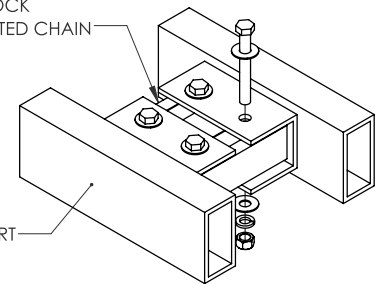
TYPICAL DOCK TO DOCK CONNECTION
