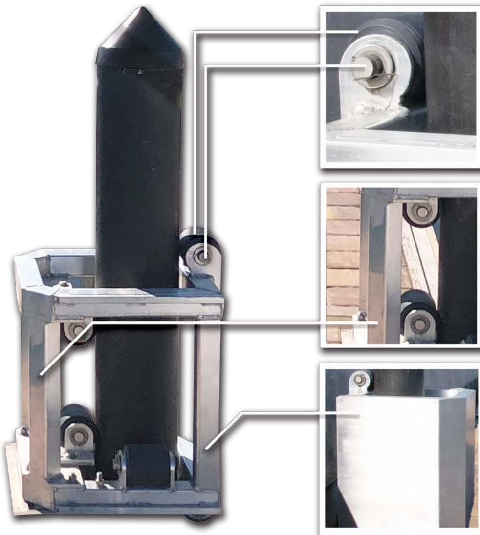
Protective Cowling Constructed with 6061-T6 Aluminum
