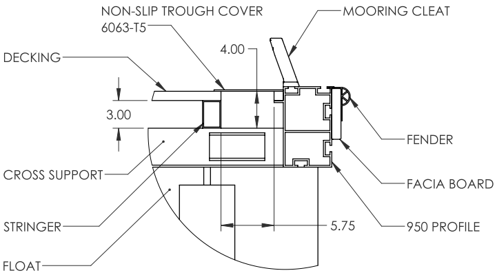
DETAIL A TYPICAL TROUGH
