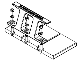
CLEAT ASSEMBLY DETAIL
