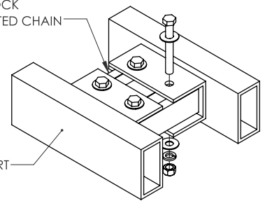
TYPICAL DOCK TO DOCK CONNECTION
