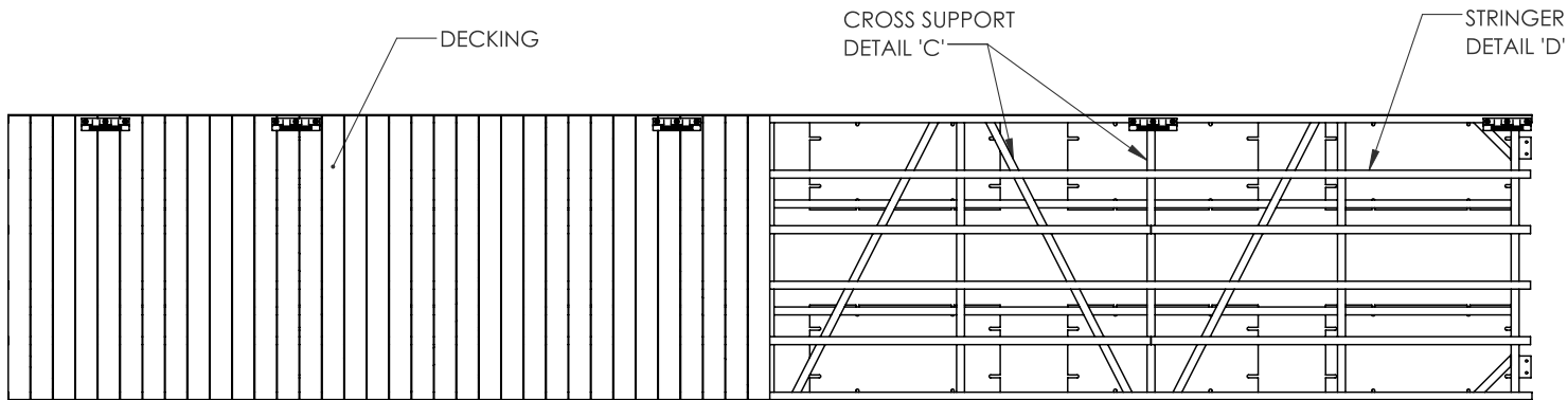
TOP VIEW
