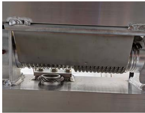
Cable Keepers
