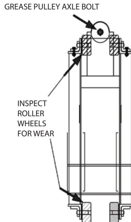
SLIDING CARRIAGE
